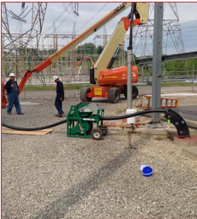
Pulling the new cable in the substation duct bank.
